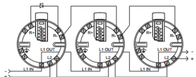
Figure 3. Wiring diagram without isolator
