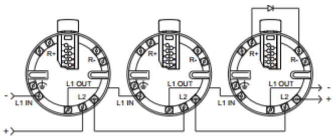
Figure 2. Wiring diagram for detectors with isolator
