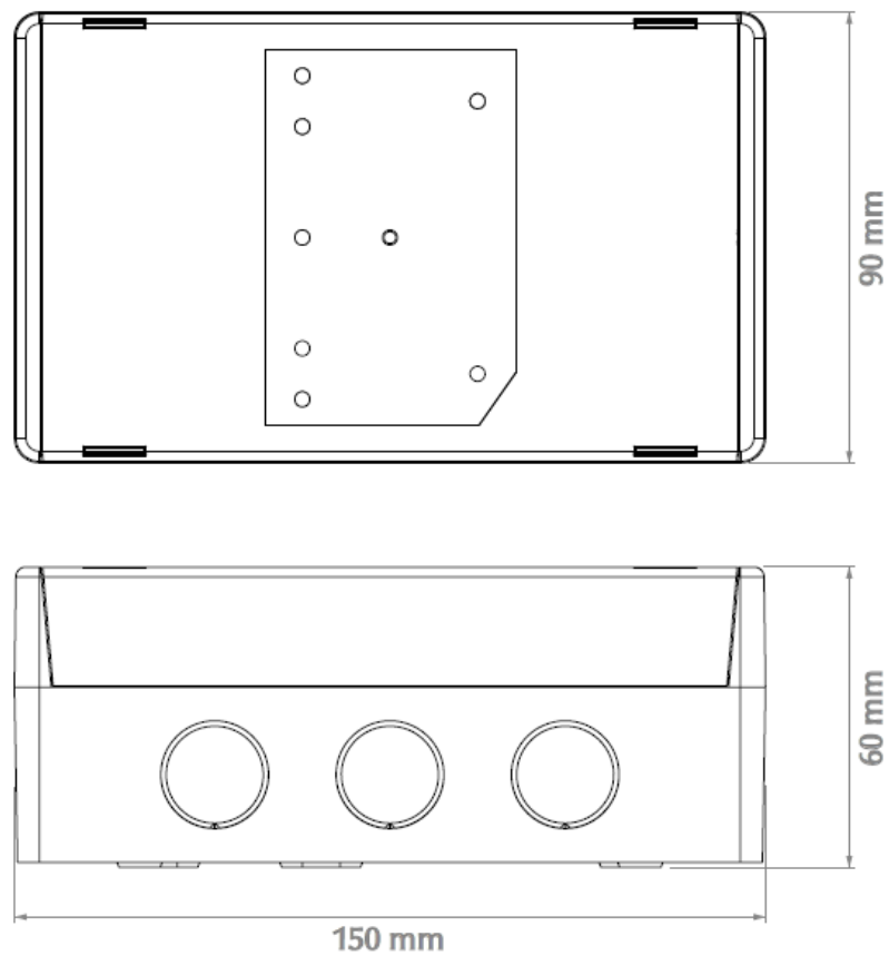
Figure 3. Dimensions
