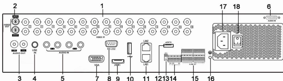
Figure 1.12 Rear Panel of DS-8132HCI-SH, DS-8132HFSI-SH and DS-8132HWSI-SH
