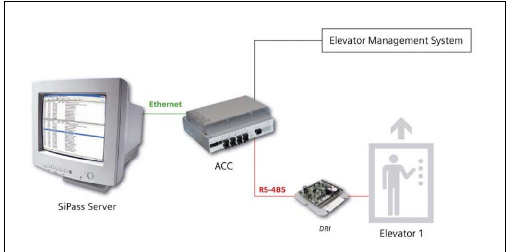
High Level Elevator Access Control Architecture
